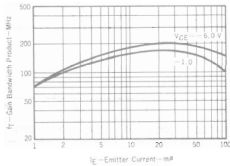
GAIN BANDWIDTH PRODUCT vs. EMITTER CURRENT
