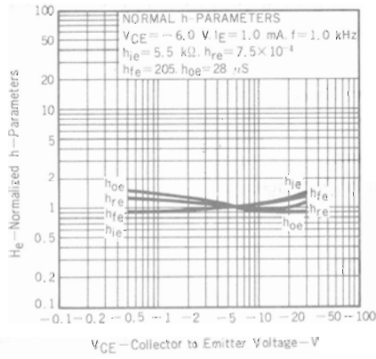
NORMALIZED h-PARAMETERS vs. COLLECTOR TO EMITTER VOLTAGE
