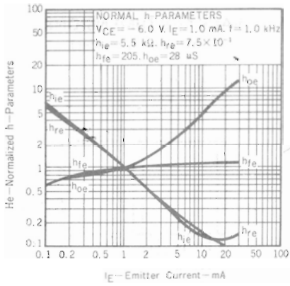
NORMALIZED h-PARAMETERS vs. EMITTER CURRENT
