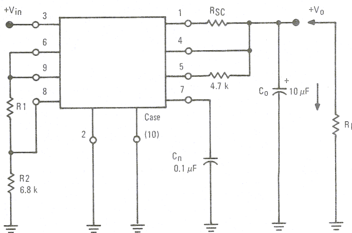
FIGURE 1 - CONNECTION FOR V_o \geq 3.5 \text{ V}
