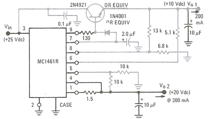
FIGURE 17 - PROVIDING TWO REGULATED OUTPUT VOLTAGES
