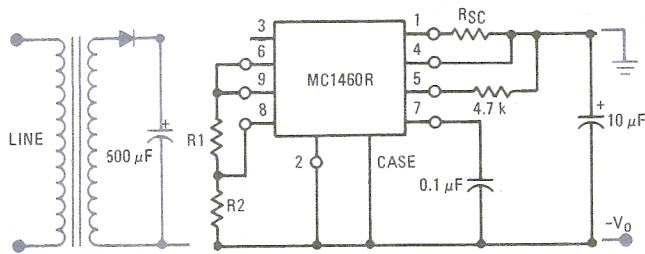
FIGURE 26 – CONNECTION FOR A NEGATIVE OUTPUT VOLTAGE
